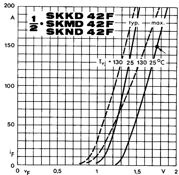
Fig. 19 Forward characteristics
