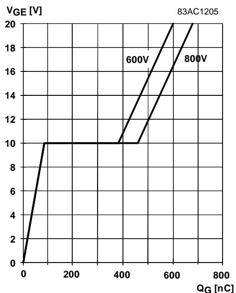
Fig. 5 Typ. gate charge characteristic
