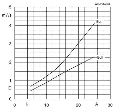
Fig. 3 Turn-on /-off energy = f(I_c)
