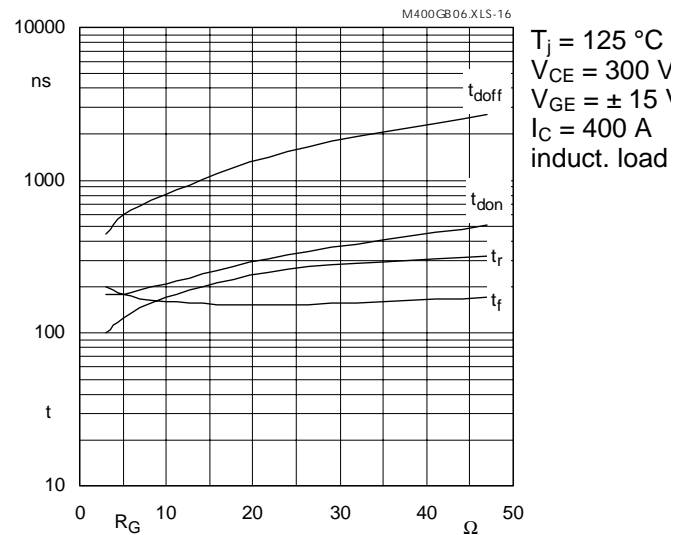
Fig. 16 Typ. switching times vs. gate resistor R_G
