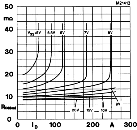
Fig. 13 On-resistance vs. drain current
