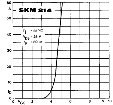
Fig. 4 Transfer characteristic
