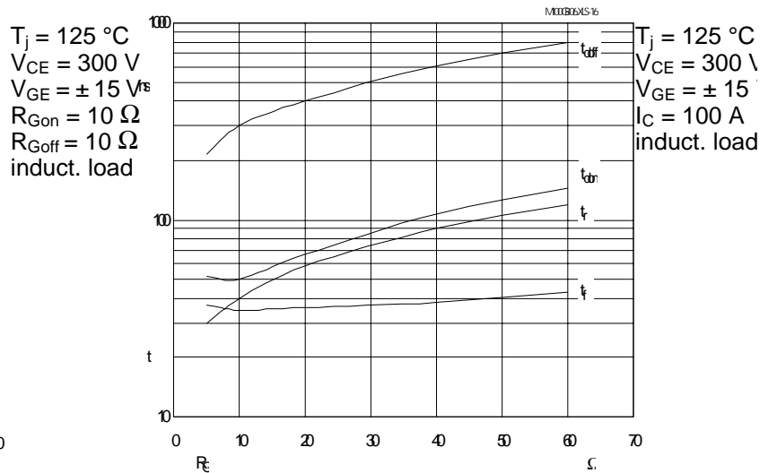
Fig. 16 Typ. switching times vs. gate resistor R_G
