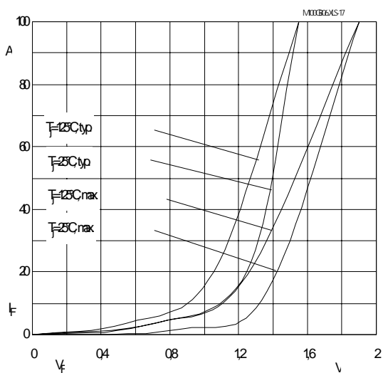
Fig. 17 Typ. CAL diode forward characteristic
