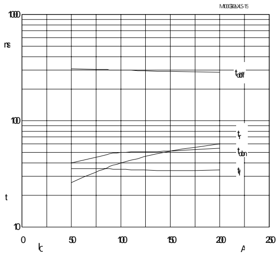
Fig. 15 Typ. switching times vs. I_C
