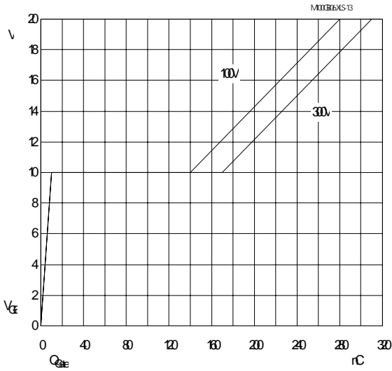
Fig. 13 Typ. gate charge characteristic
